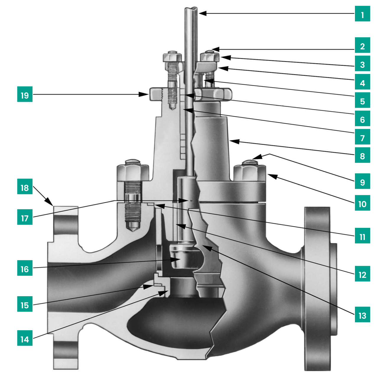
Standard Construction
